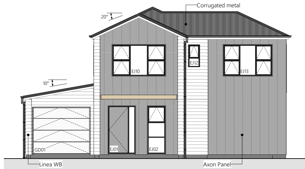
1 South Elevation 1:100
