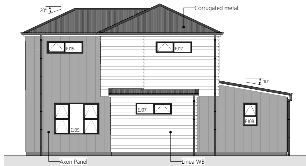
3 North Elevation 1:100
