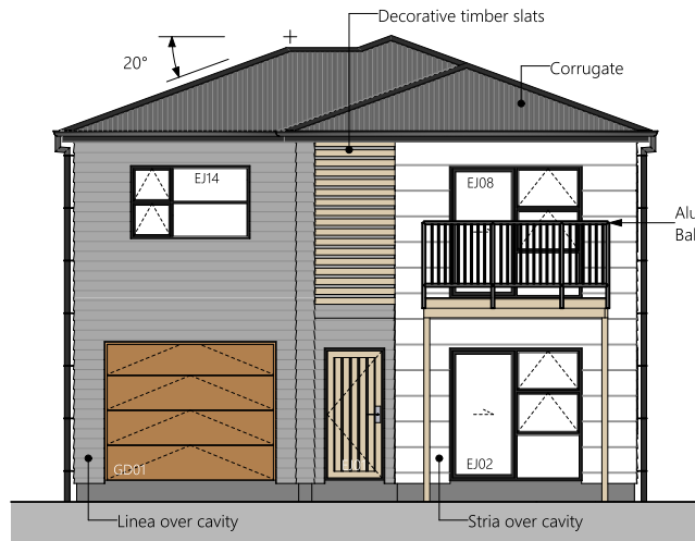
1 West Elevation
