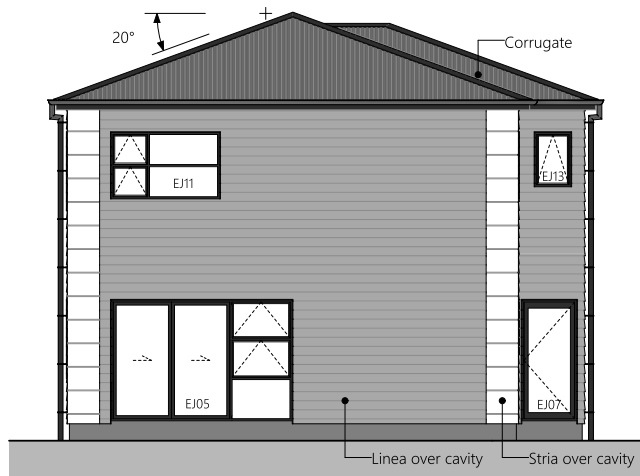
3 East Elevation
