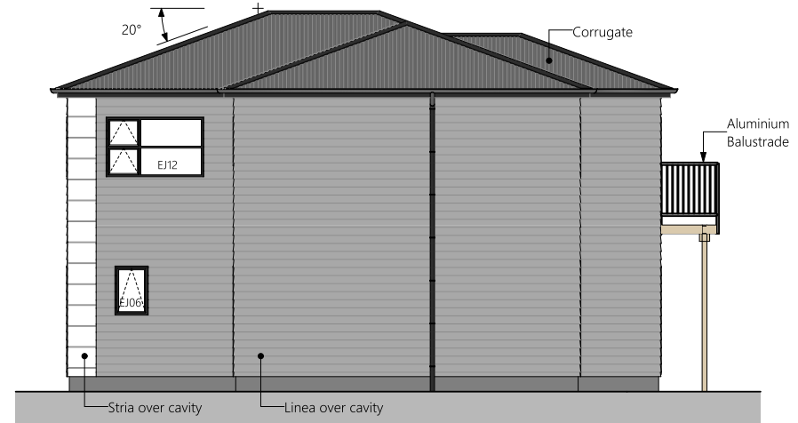
4 North Elevation
