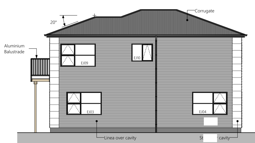
2 South Elevation
