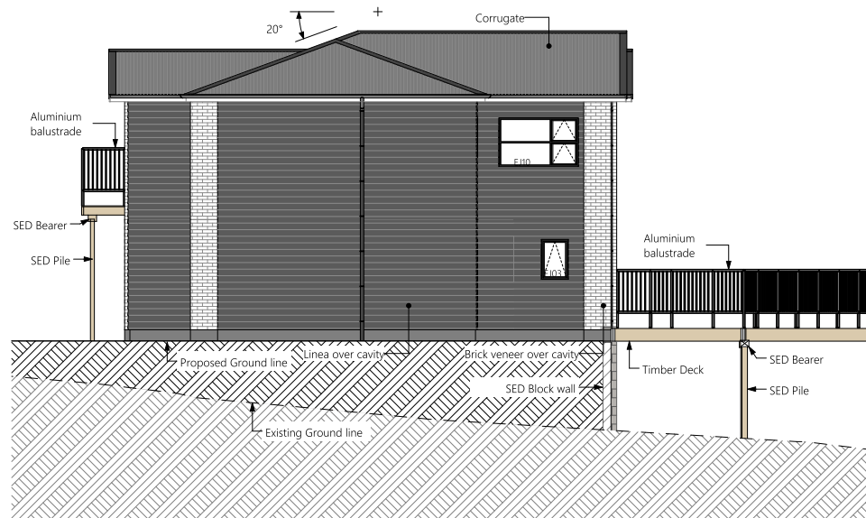
4 Lot 06 North Elevation
