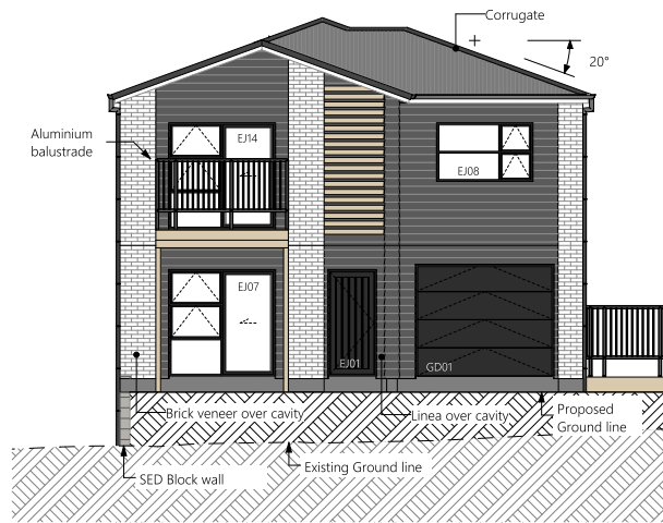
1 Lot 06 East Elevation
