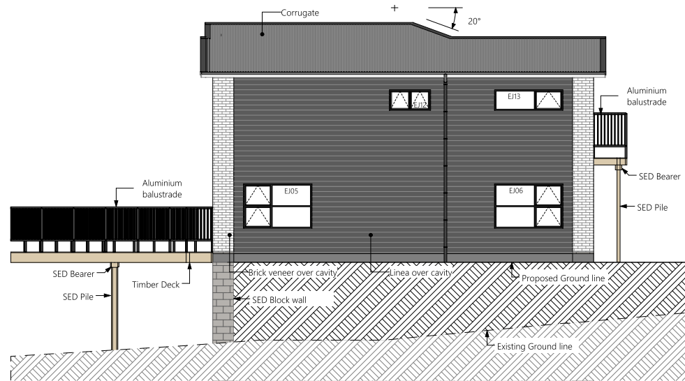
2 Lot 06 South Elevation
