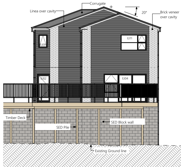
3 Lot 06 West Elevation
