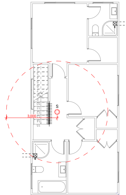
Upper Electrical Plan
