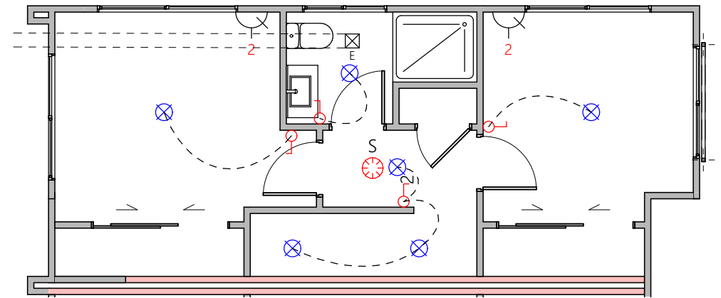
Upper Electrical Plan
