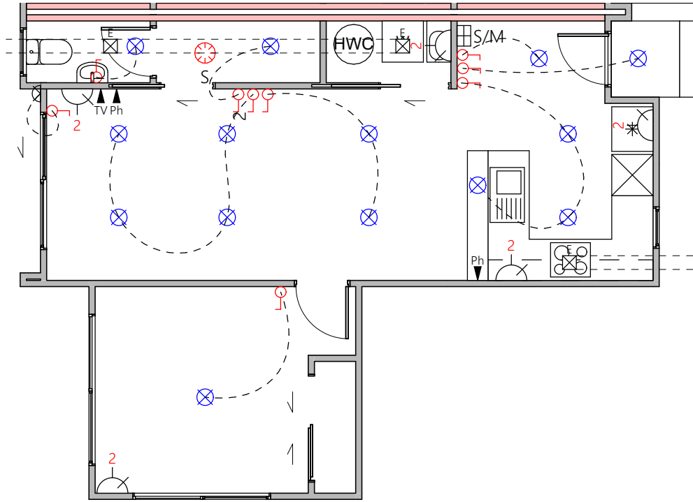
Lower Electrical Plan
