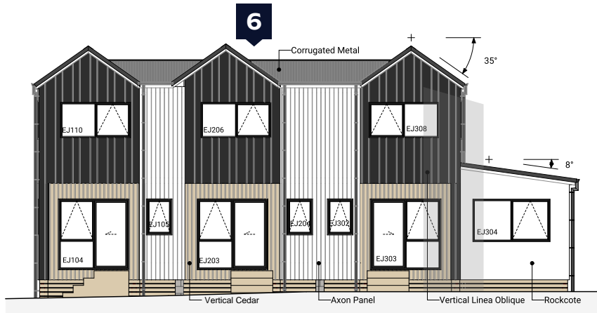
3 South West Elevation
