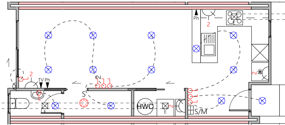
Lower Electrical Plan
