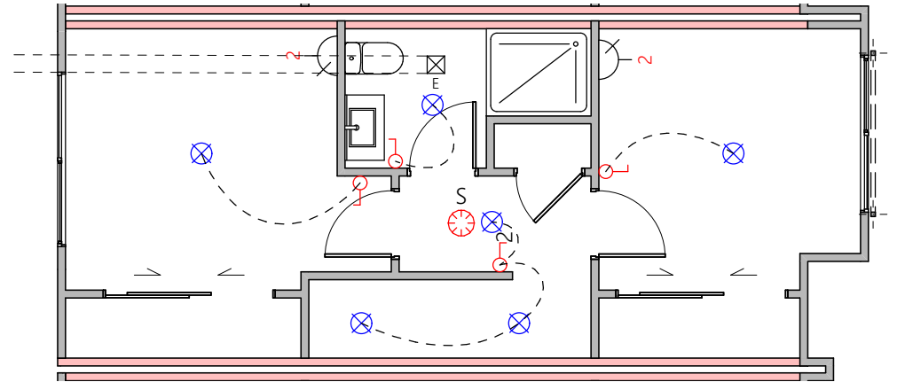
Upper Electrical Plan
