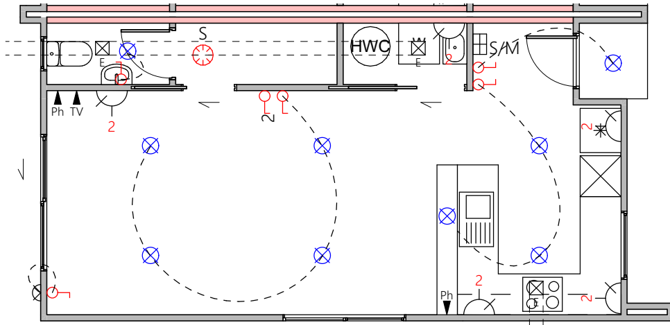
Lower Electrical Plan
