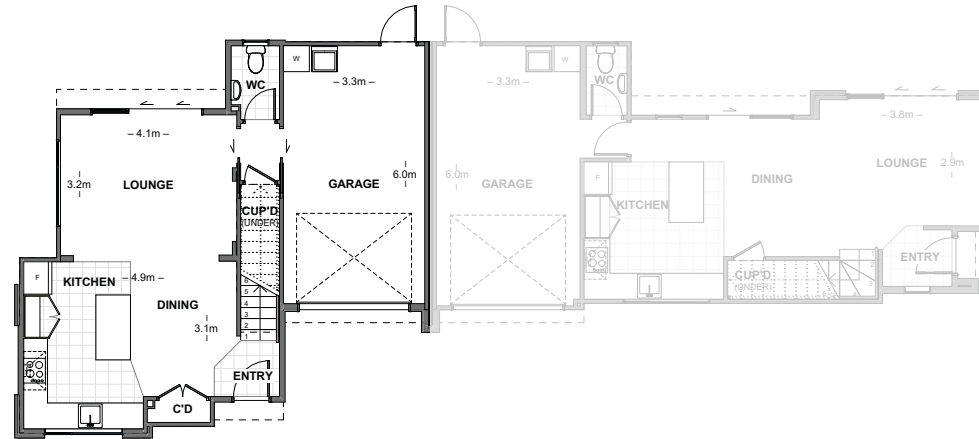
LOWER LEVEL FLOOR PLAN 64.98m 2
