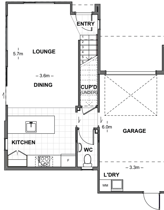
LOWER LEVEL FLOOR PLAN 61.55m 2
