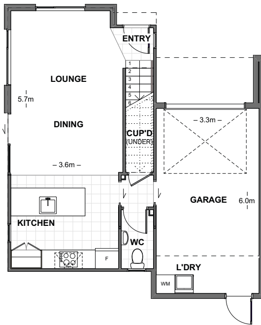
LOWER LEVEL FLOOR PLAN 61.92m 2
