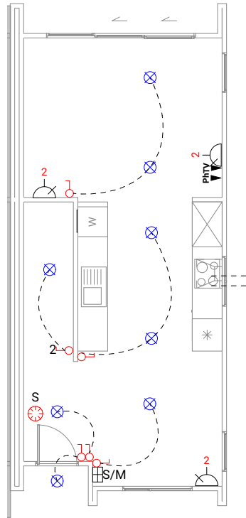
Lower Electrical Plan
