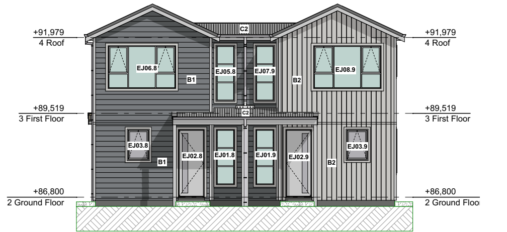
4 South-West Elevation
